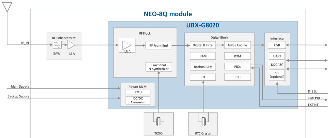
Figure 1: NEO-8Q block diagram
